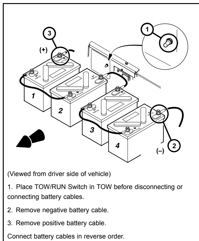
422 Figure 2 Battery Cable Removal – 4x12-Volt Battery Configuration
