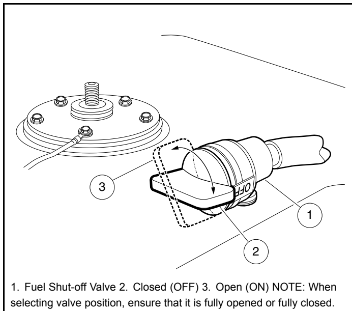
614 Figure 24 Fuel Shut-off Valve
